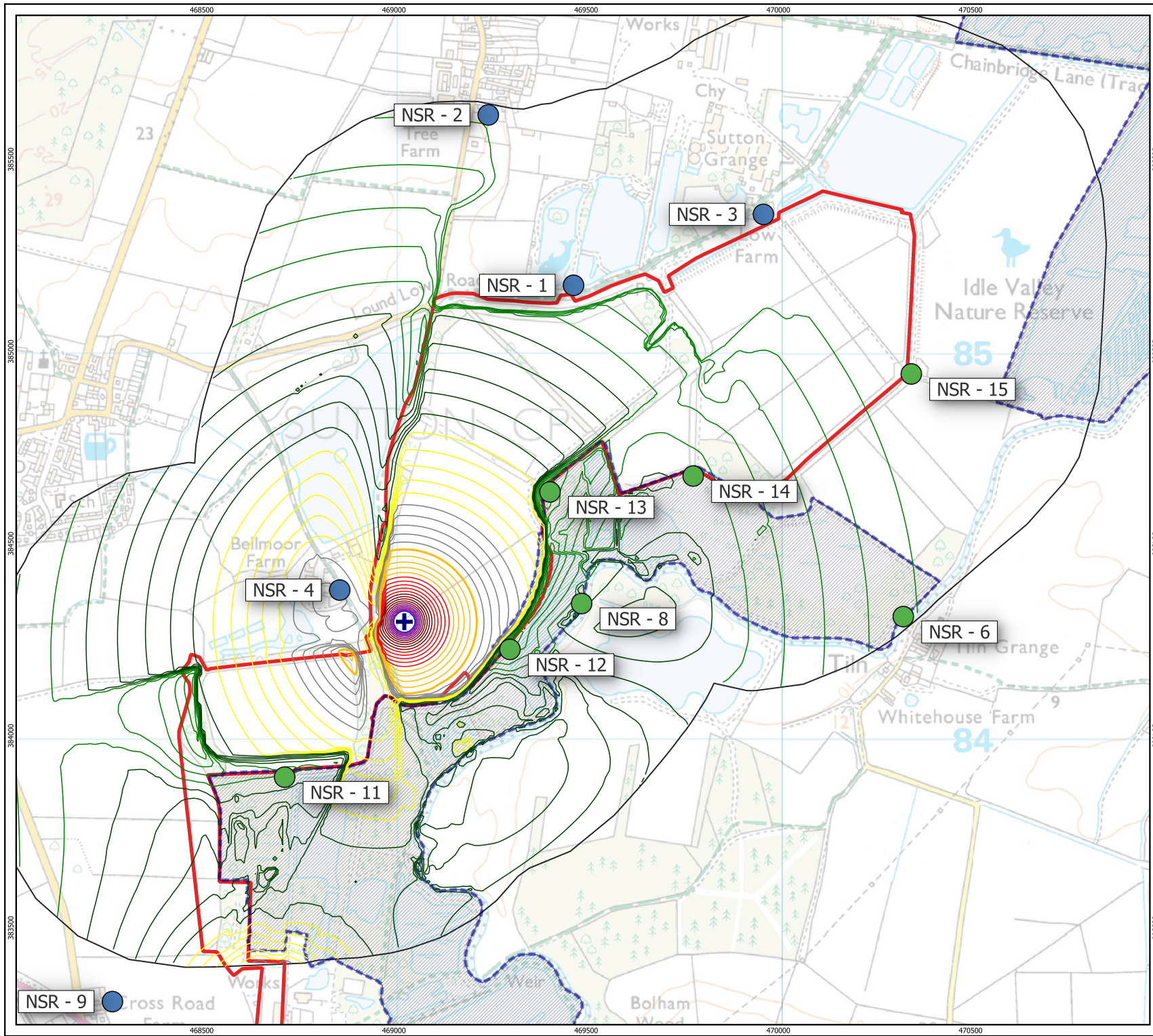
Figure 12.34 Embankment Removal: HRP2
