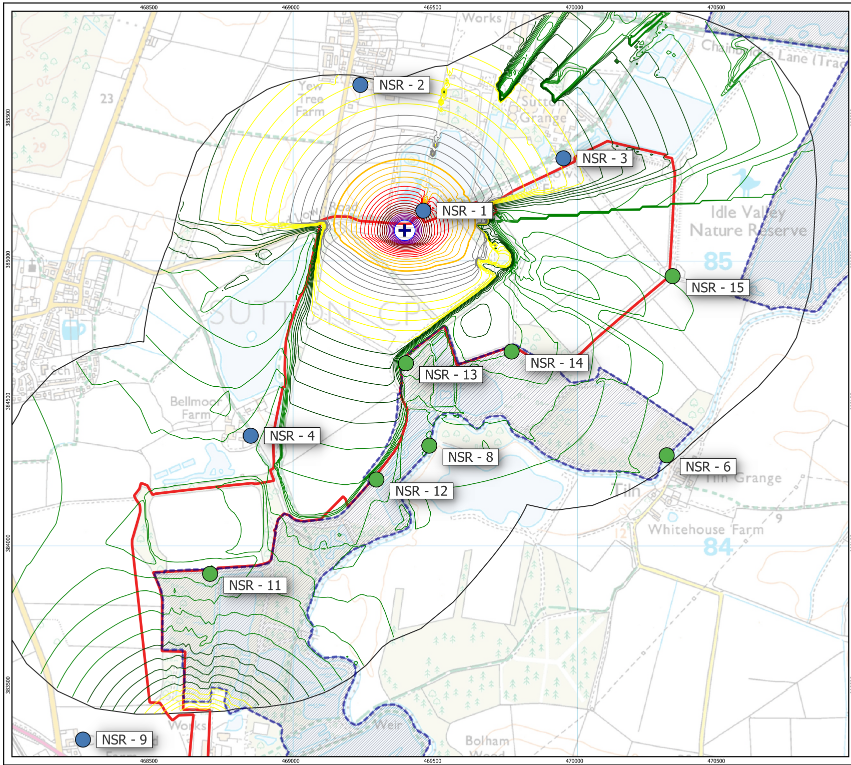
Figure 12.37 Embankment Removal: HRP5
