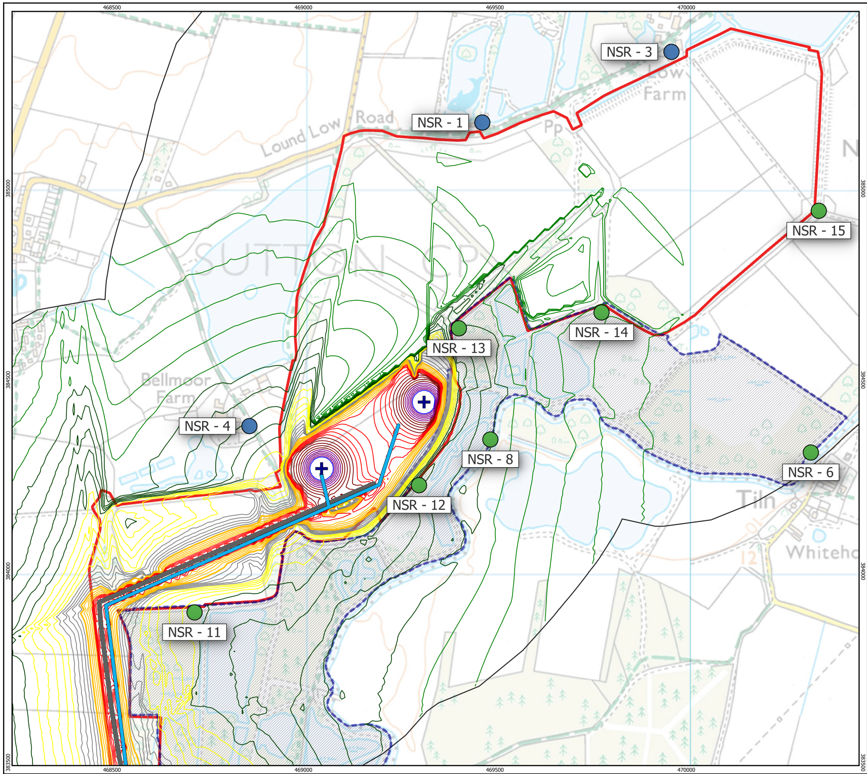
Figure 12.4 Extraction Scenario 2 - Daytime
