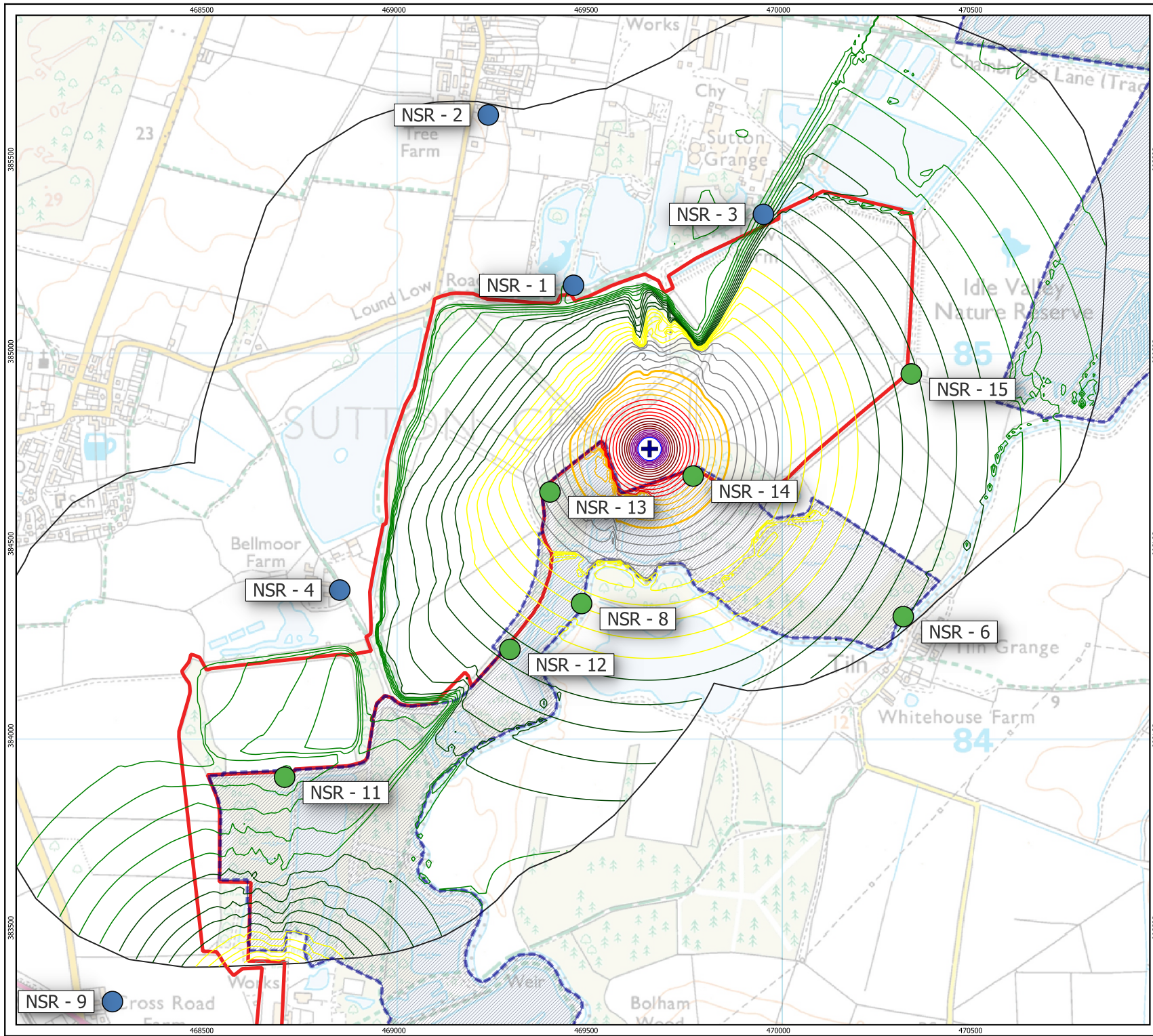
Figure 12.40 Embankment Removal: LRP2
