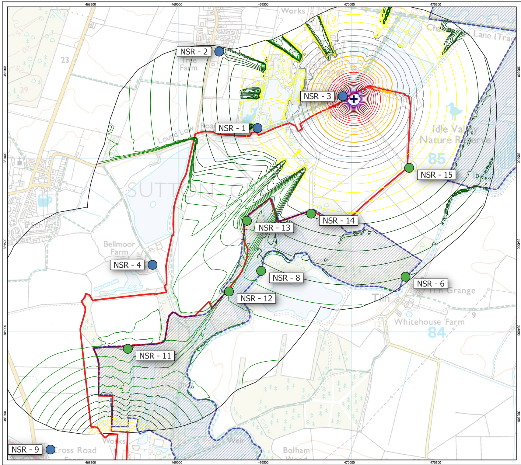
Figure 12.43 Embankment Removal: LRP5
