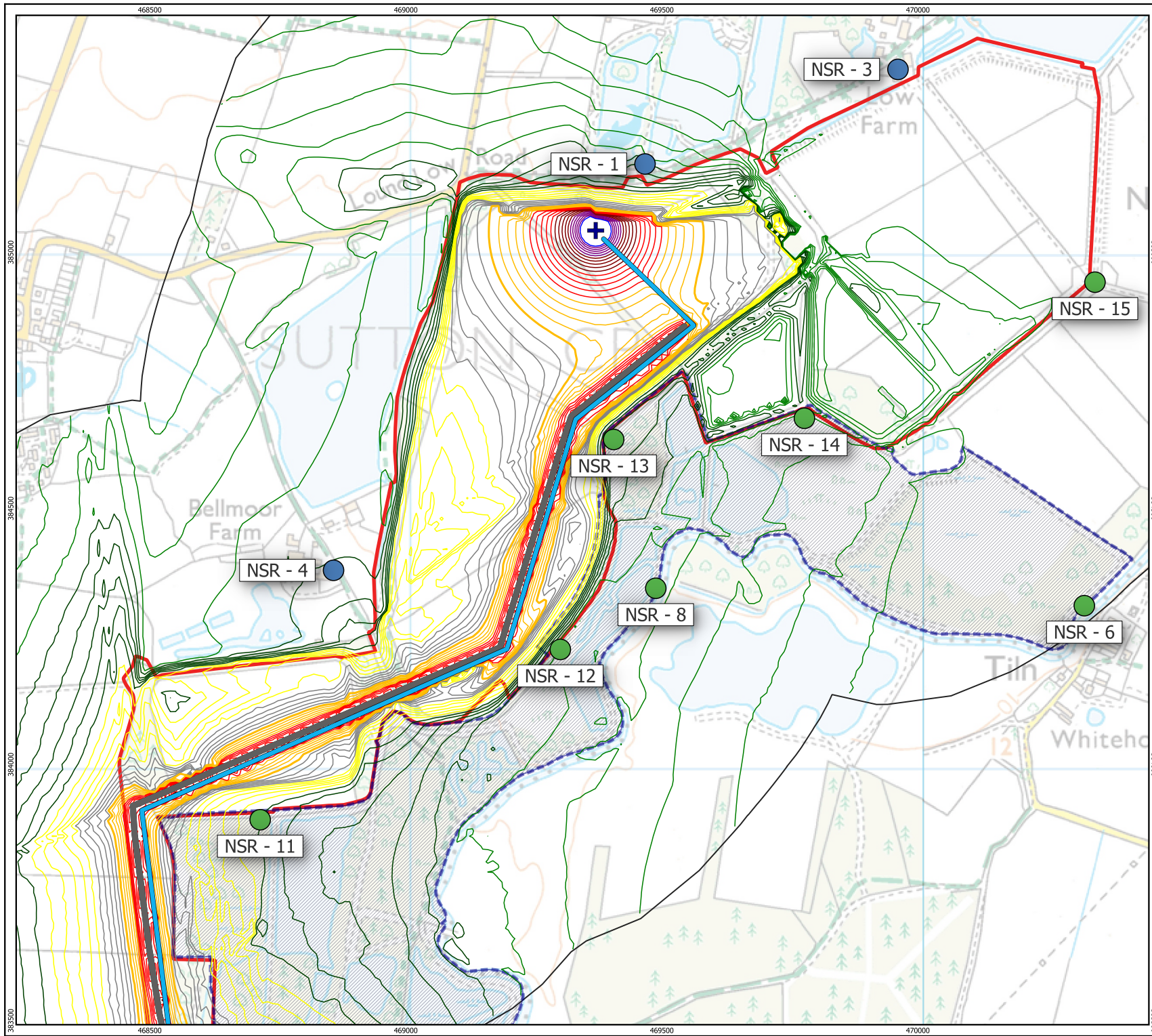
Figure 12.7 Extraction Scenario 5 - Daytime
